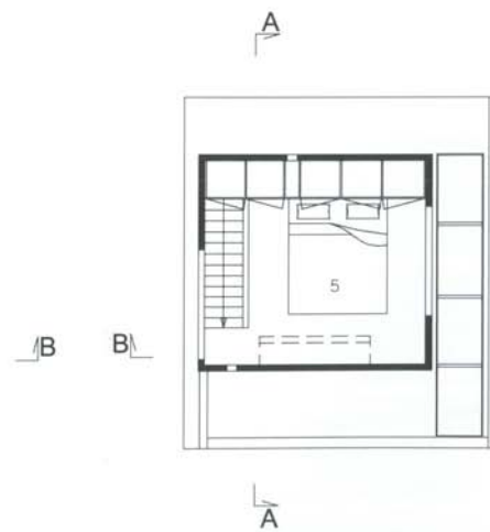
Third floor plan Plano del tercer piso
